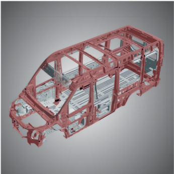
Frontal Crash Compliant Monocoque Structure
