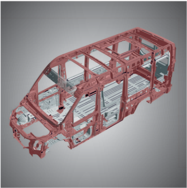
Frontal Crash Compliant Monocoque Structure
