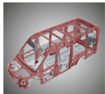
Frontal Crash Compliant Monocoque Structure
